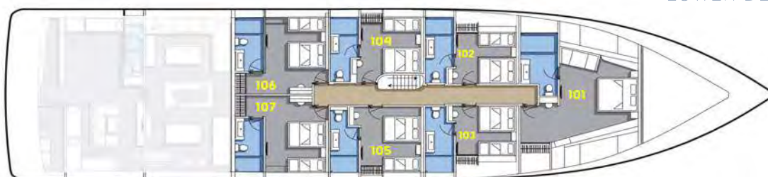
LOWER DECK
